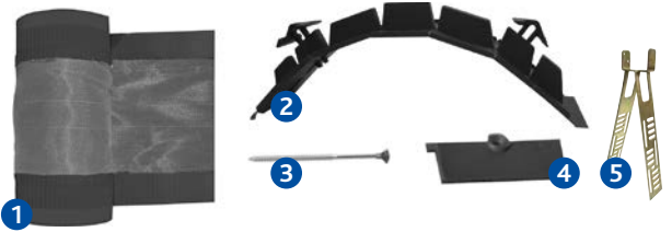
Dry Half Round Non-Interlocking Ridge - Typical Detail
