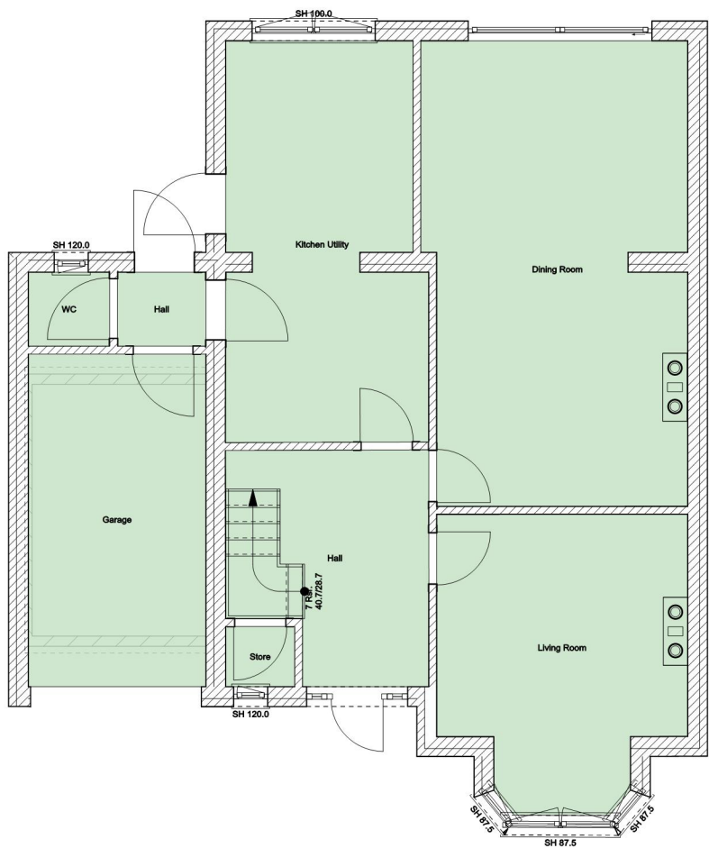
Ground Floor Exsiting Floor Plan
