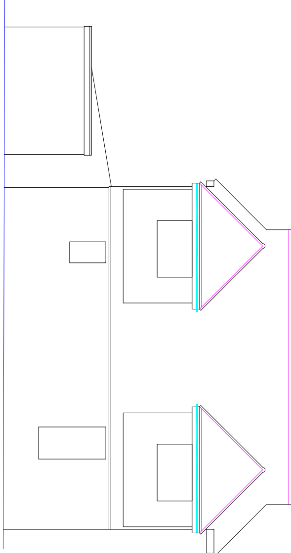
EXISTING NORTH ELEVATION 1:100
