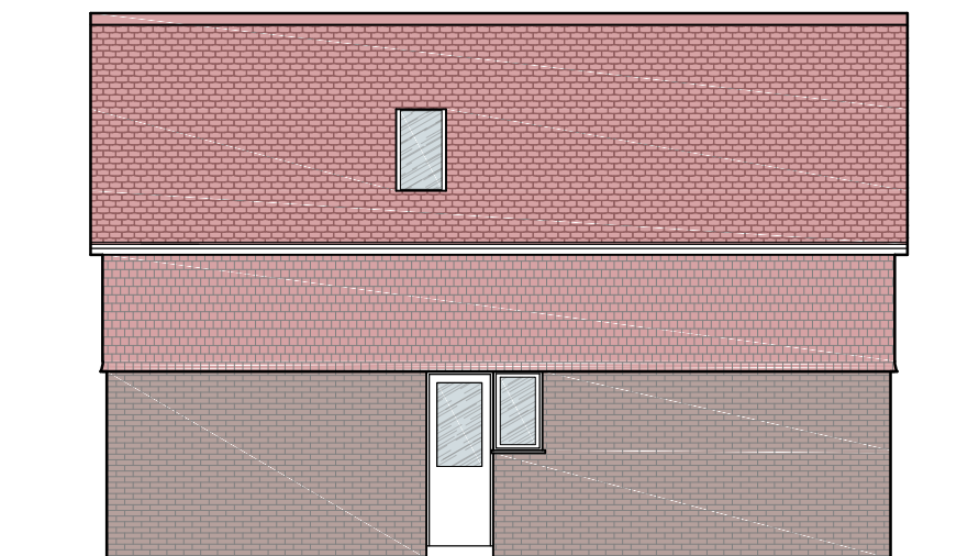
200 F PROPOSED SOUTHERN ELEVATION 1:100 (NO CHANGE TO ELEVATION)
