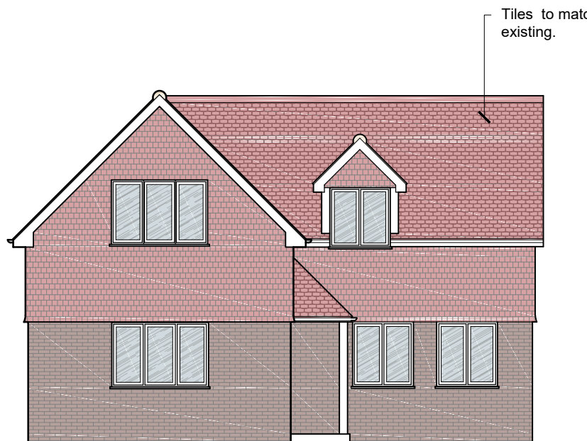
200 E PROPOSED EASTERN ELEVATION 1:100
