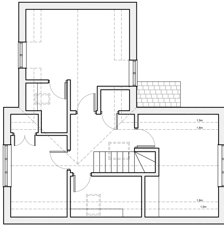
100 C PROPOSED FIRST FLOOR PLAN 1:100
