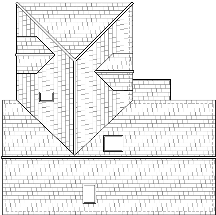
100 B EXISTING ROOF PLAN 1:100
