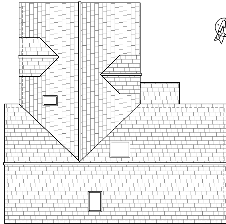
100 D PROPOSED ROOF PLAN 1:100
