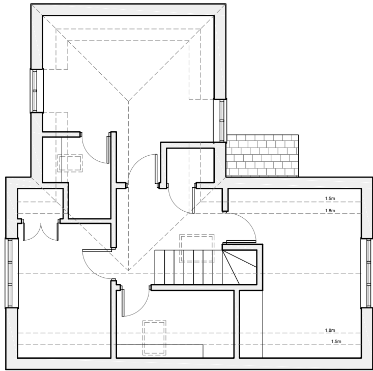
100 A EXISTING FIRST FLOOR PLAN 1:100
