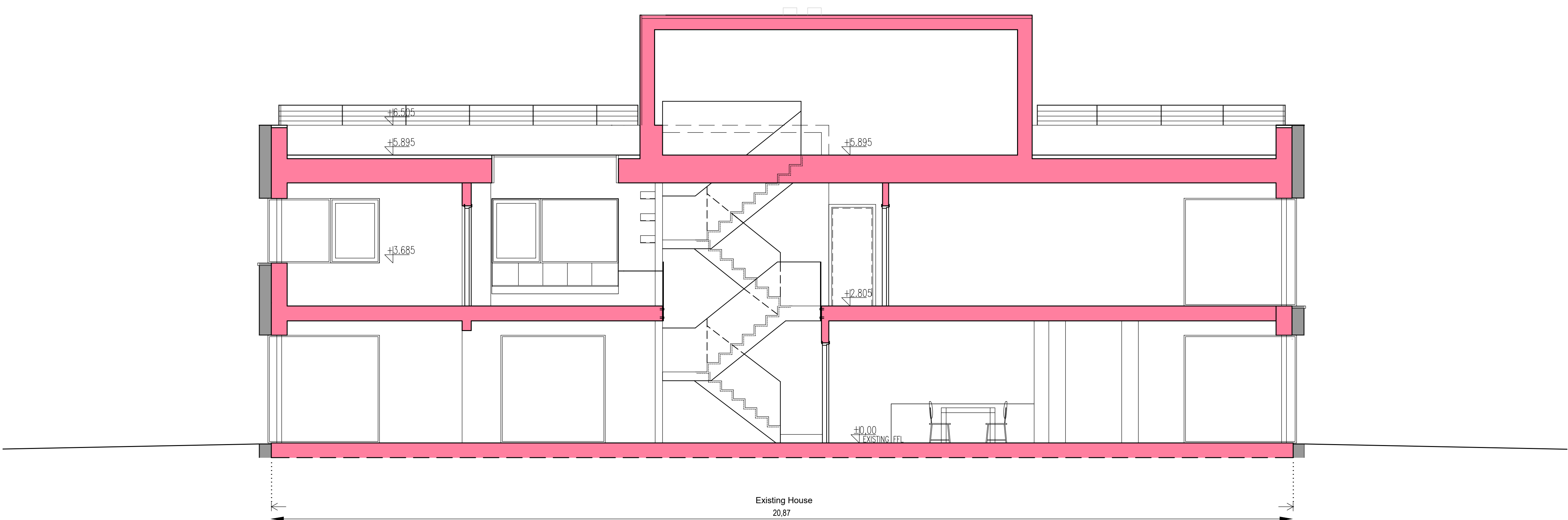
SECTION EE
