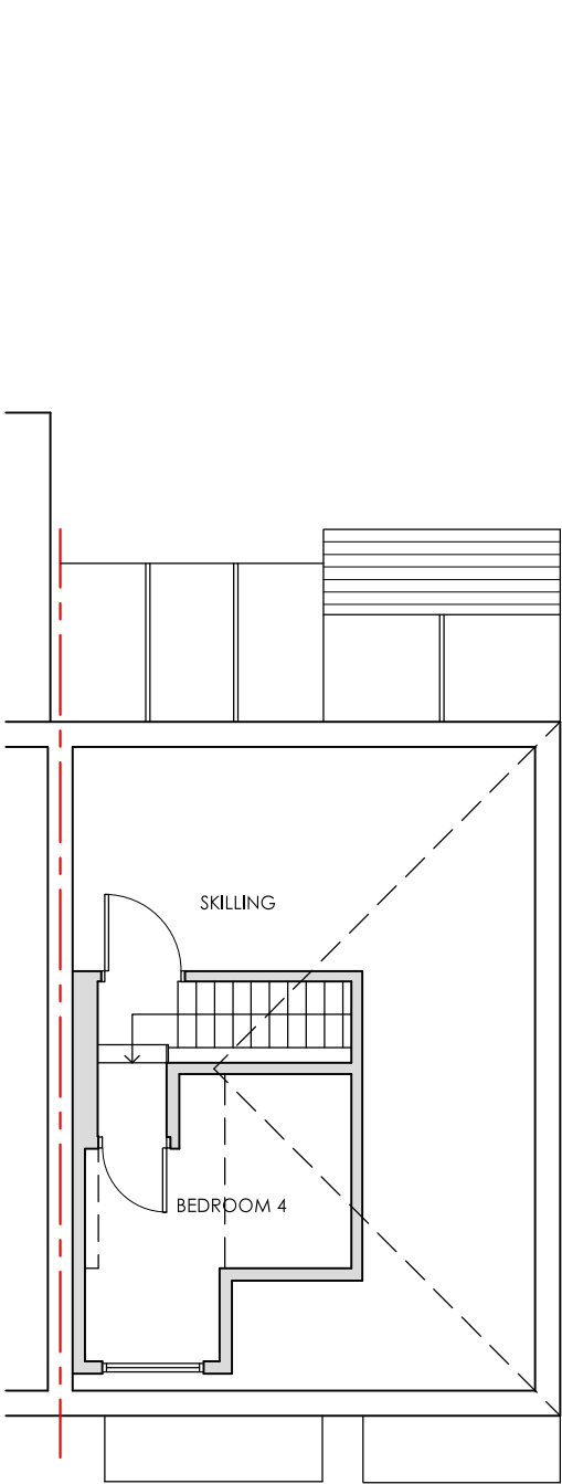
EXISTING SECOND FLOOR PLAN 1:100
