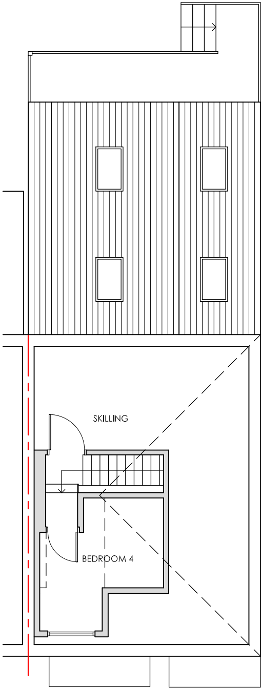
PROPOSED SECOND FLOOR PLAN 1:100
