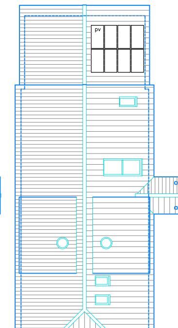
PROPOSED ROOF LEVEL
