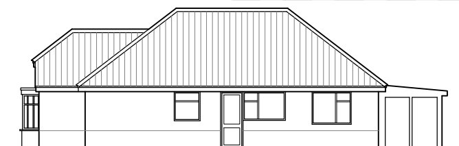
EXISTING SIDE ELEVATION (SOUTH)
