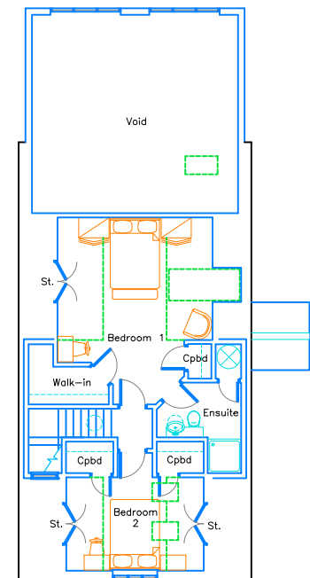
PROPOSED 1ST FLOOR
