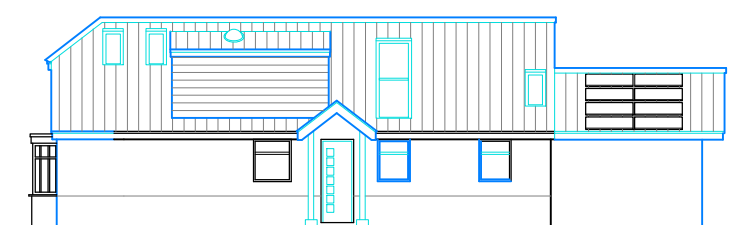
PROPOSED SIDE ELEVATION (SOUTH)
