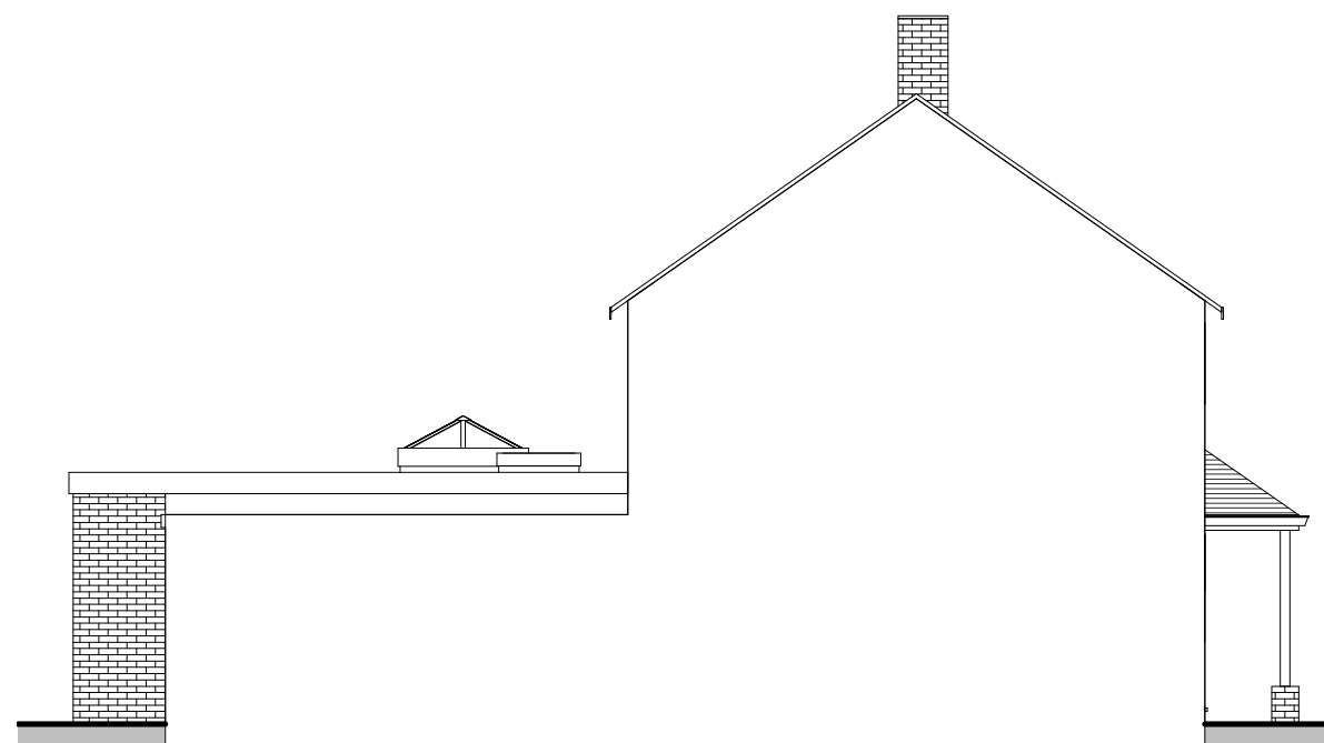
Proposed NW Elevation
