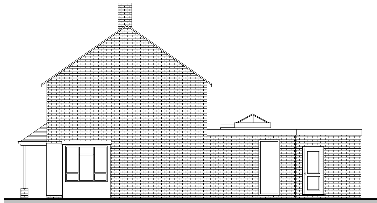
Proposed SE Elevation
