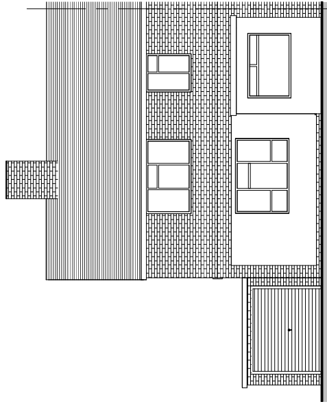
Proposed South Elevation 1 : 100
