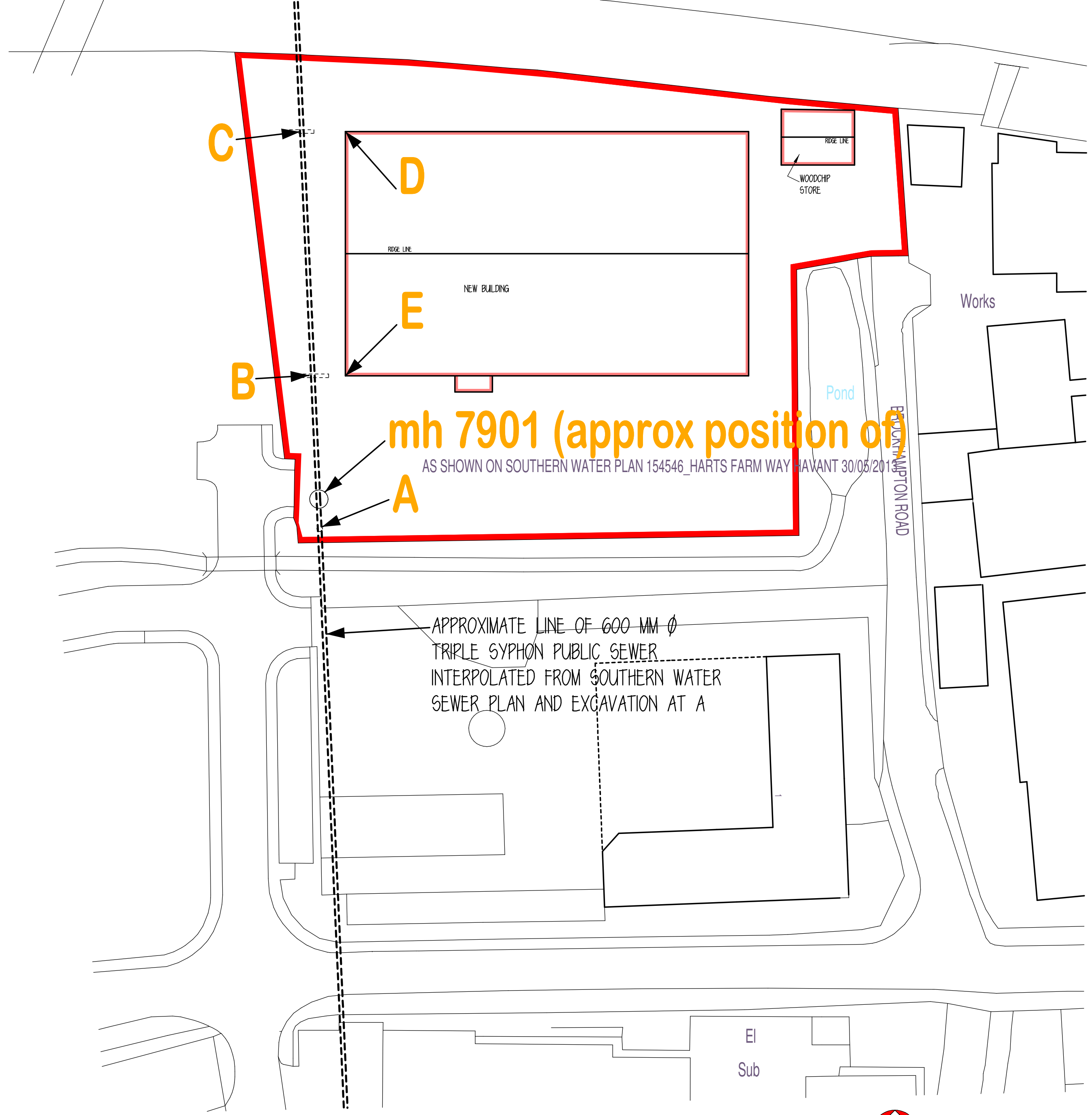
BLOCK PLAN 1:500
