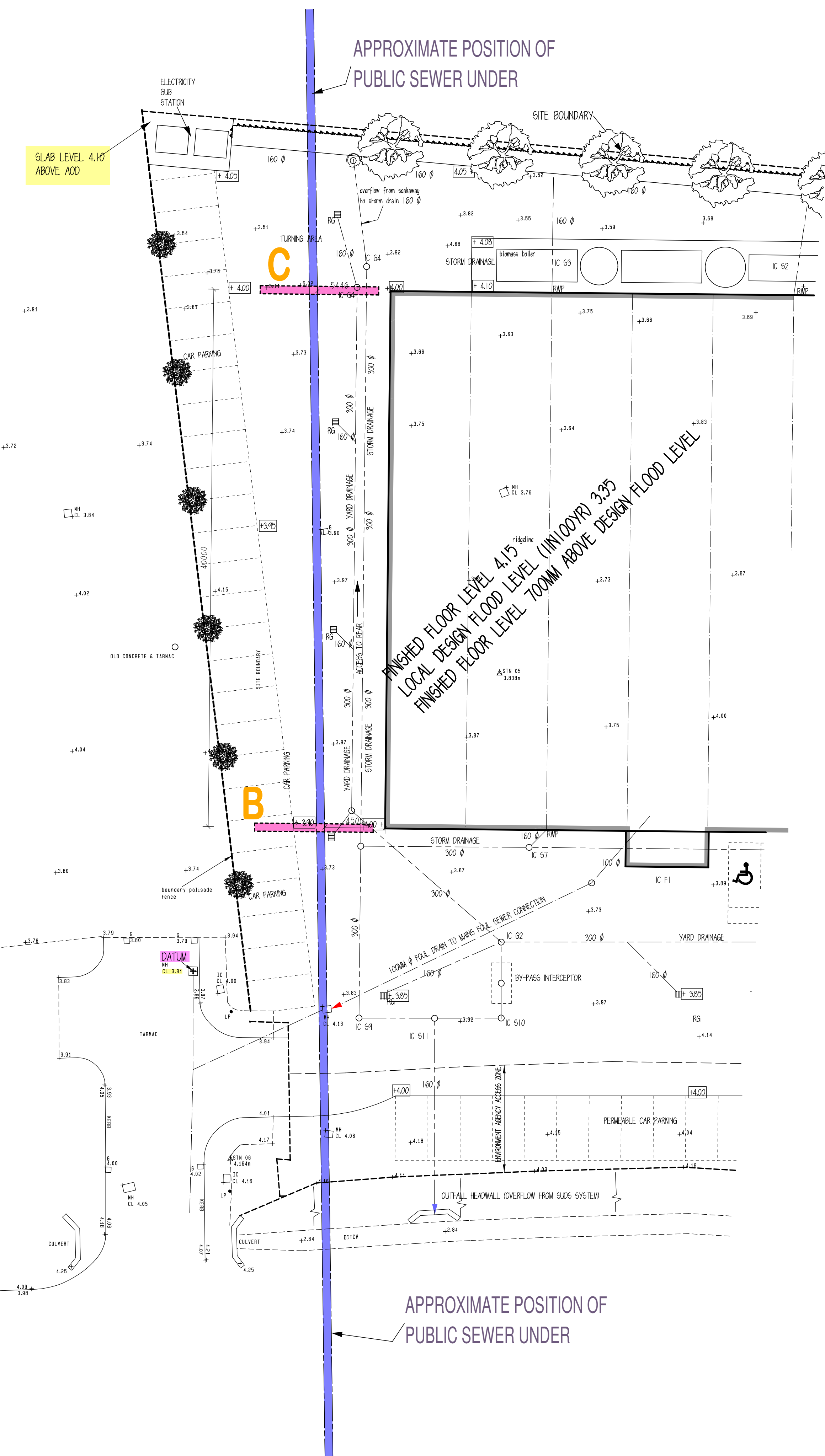
BLOCK PLAN 1:200
