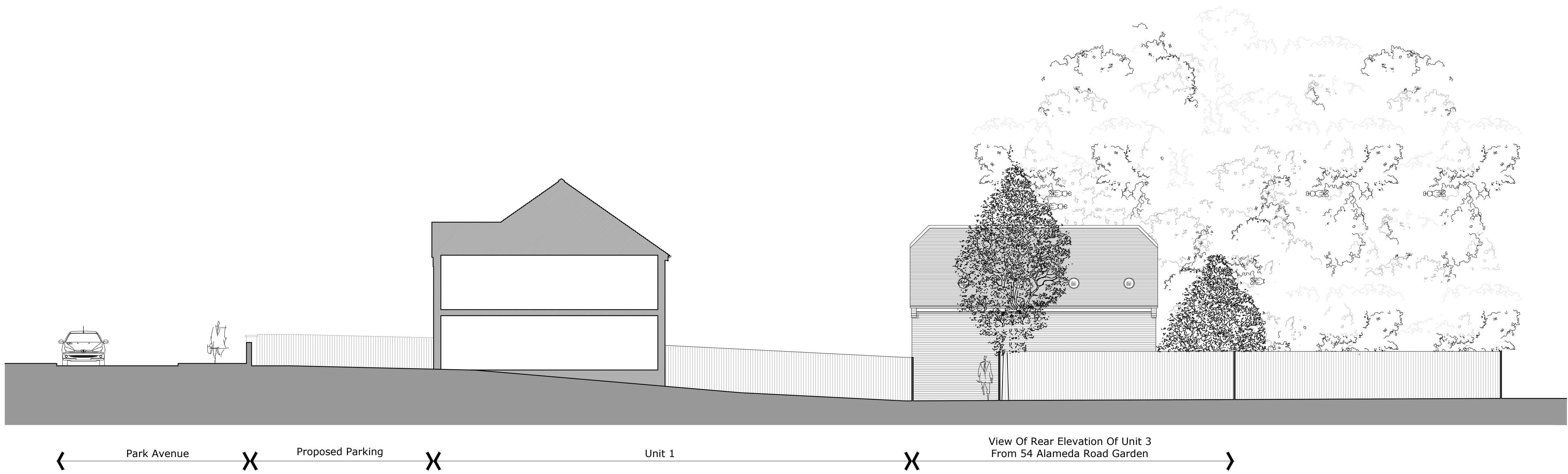
Proposed Site Section B-B 1:100
