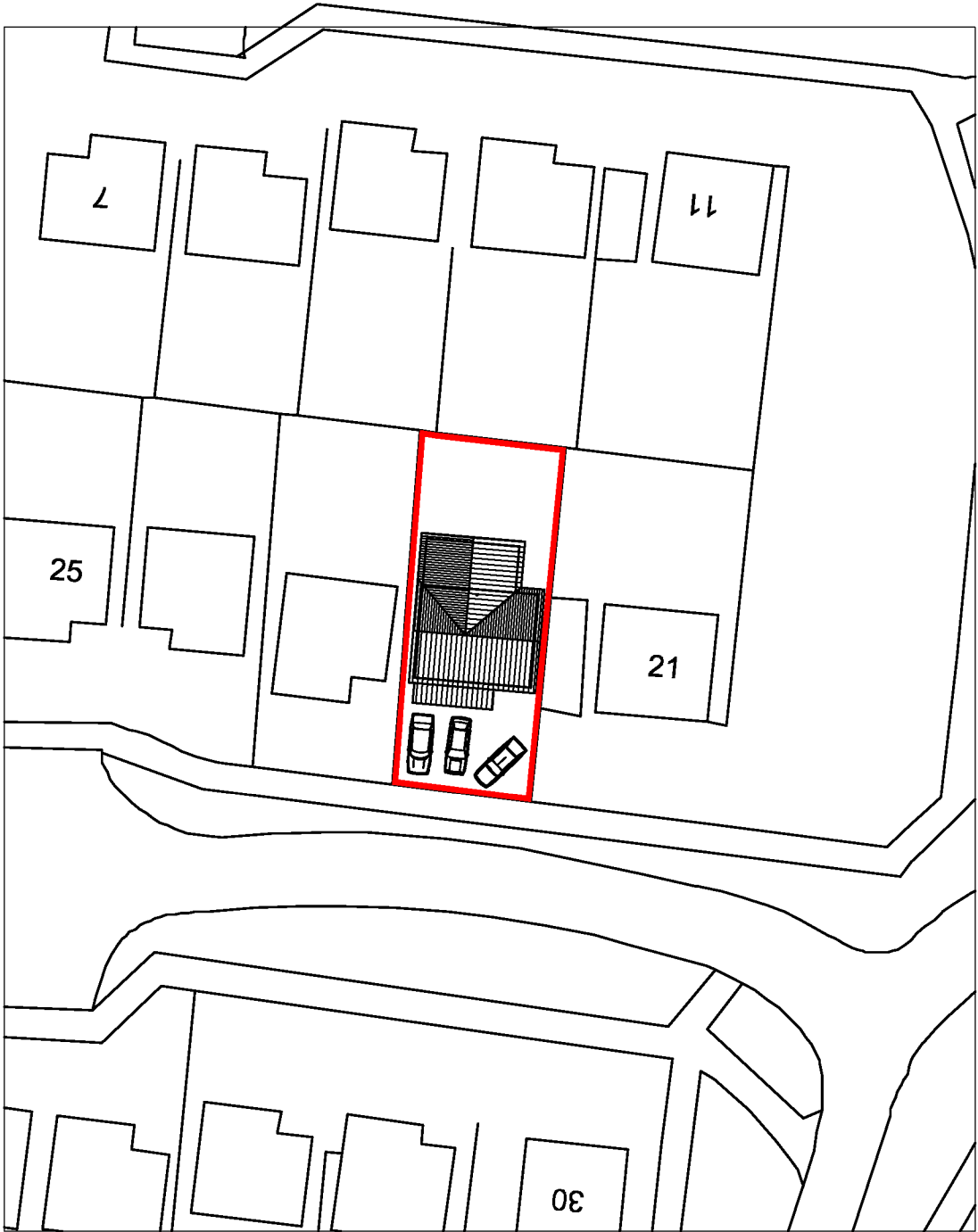
Block Plan: 1:500
