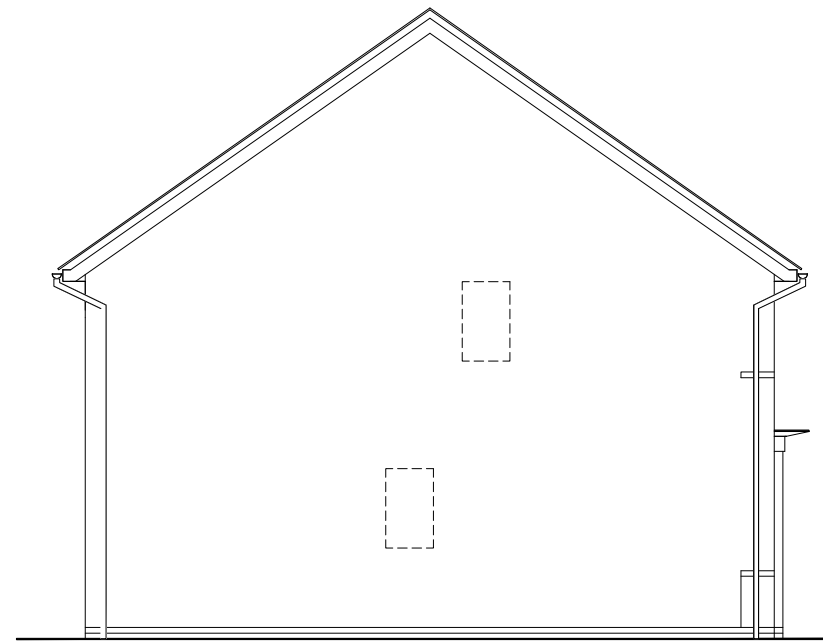
SIDE ELEVATION 1
