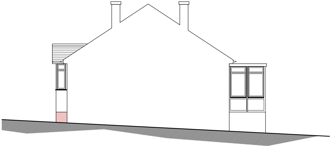
PARTY WALL ELEVATION 1:100 SCALE
