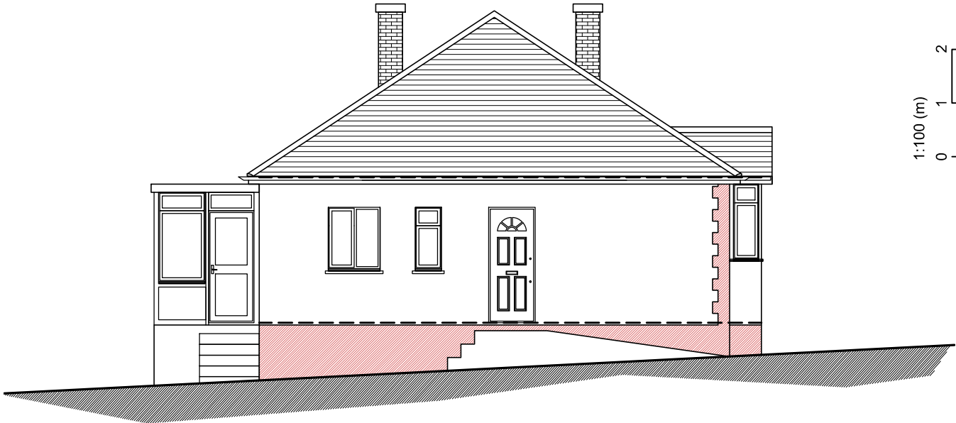
FLANK ELEVATION 1:100 SCALE
