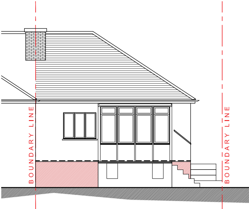
REAR ELEVATION 1:100 SCALE
