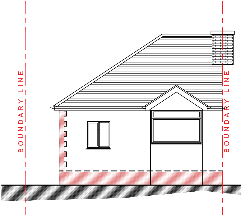
FRONT ELEVATION 1:100 SCALE
