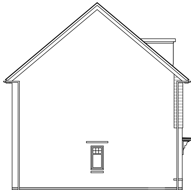
SIDE ELEVATION 1
