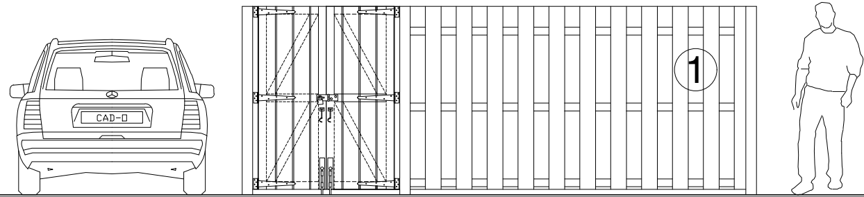
BIN STORE NORTH ELEVATION
