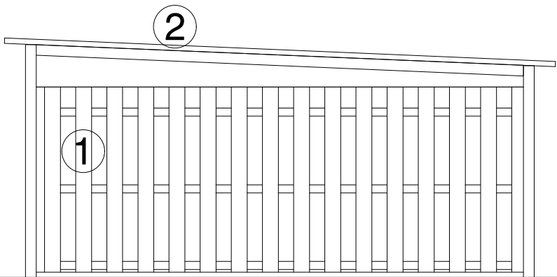
CYCLE STORE EAST ELEVATION
