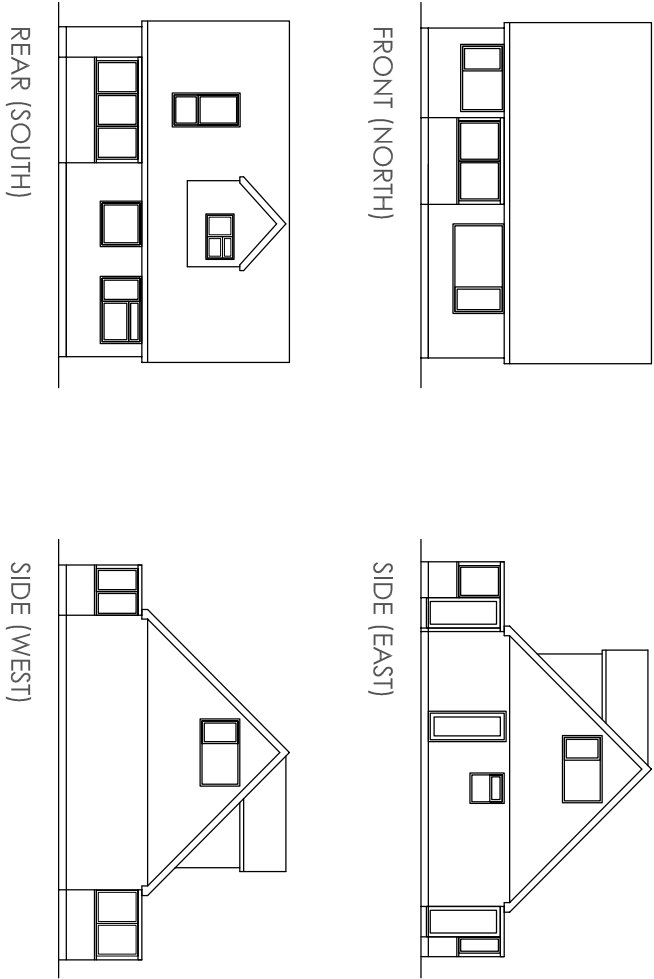
EXISTING ELEVATIONS 1:200
