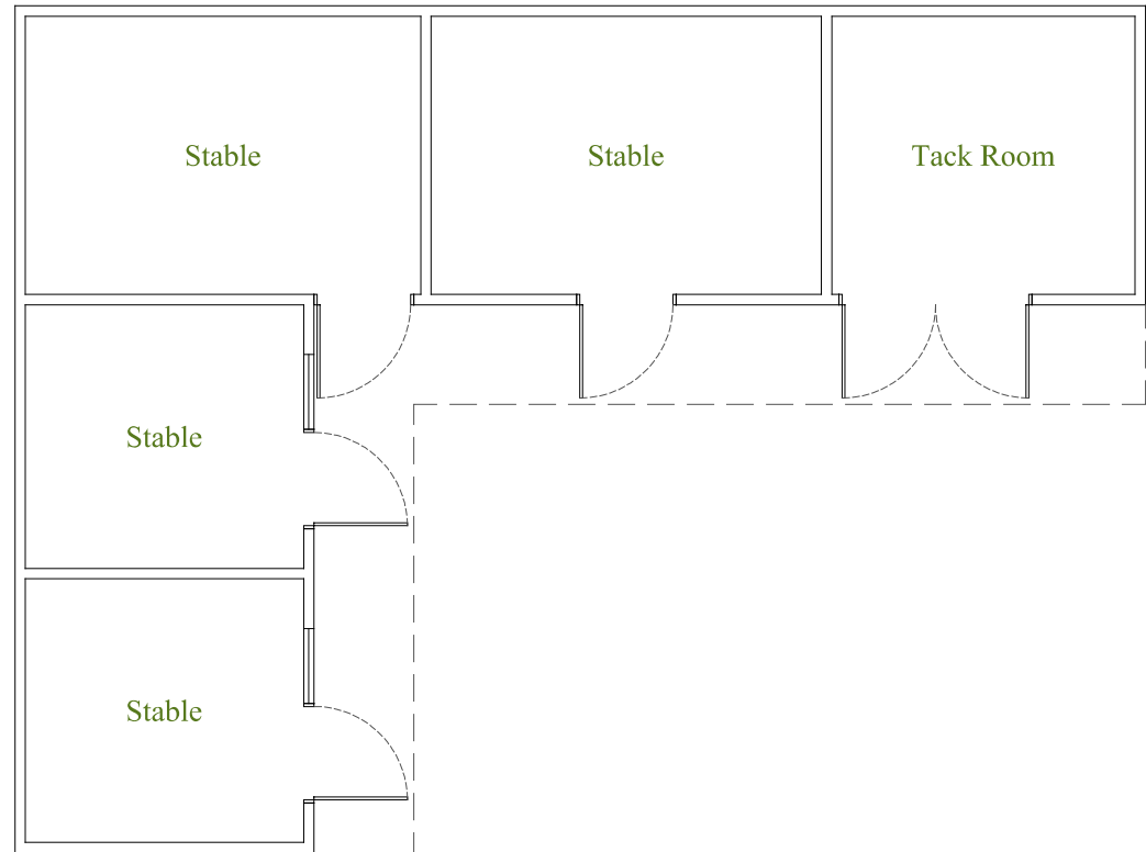
Floor Plan 1:100
