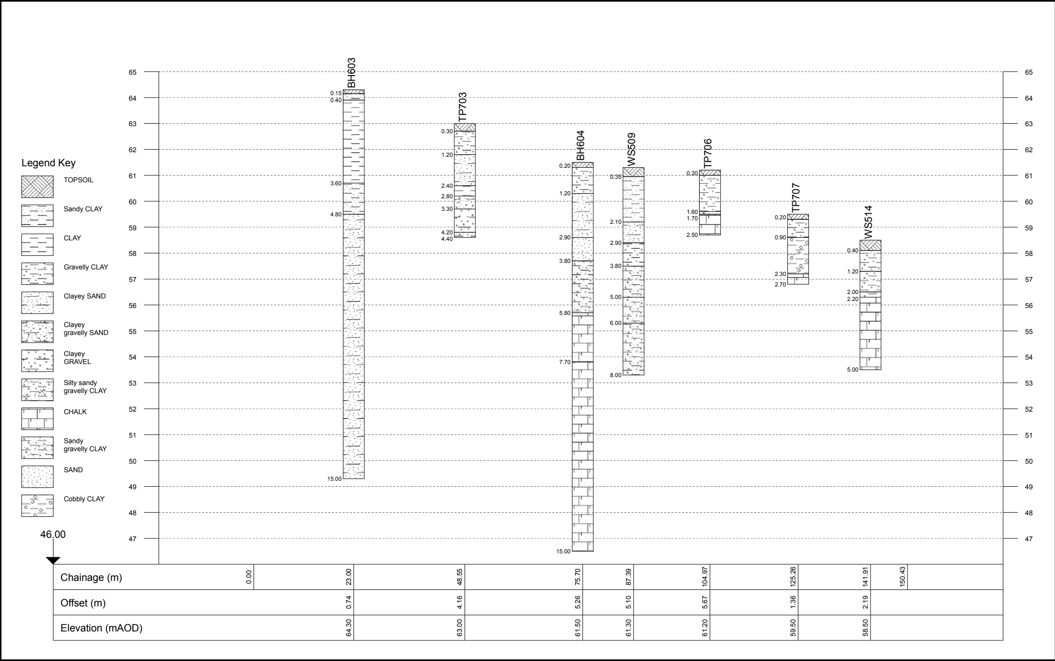
Figure 9 Section BH603 to WS514
