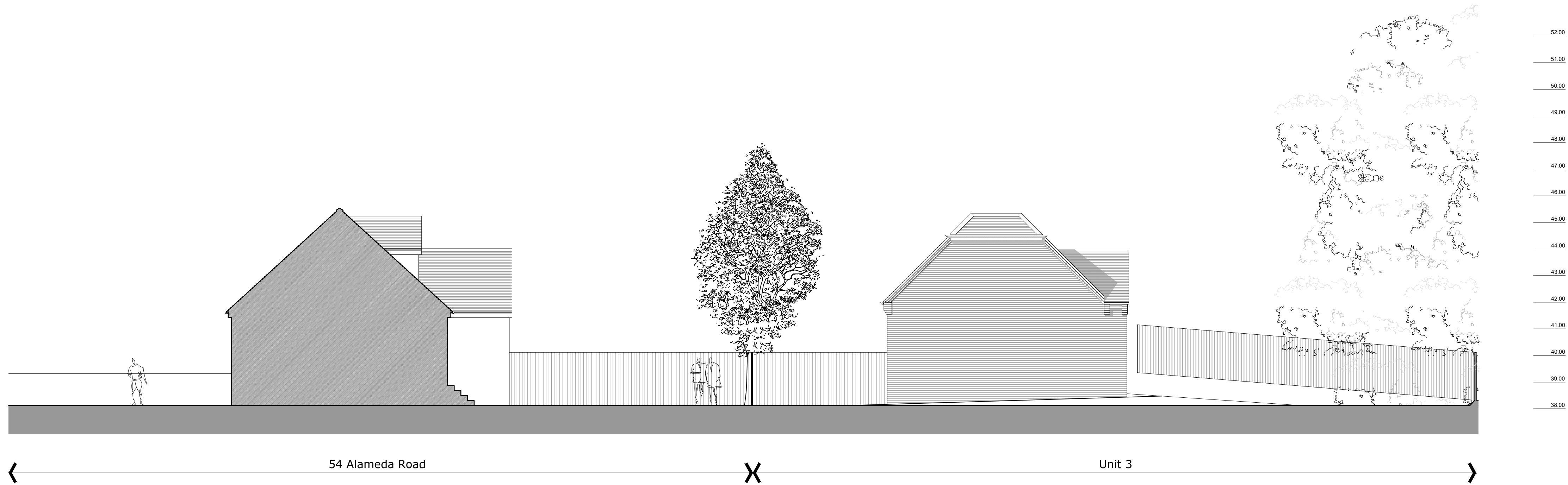
Proposed Site Section A-A 1:100
