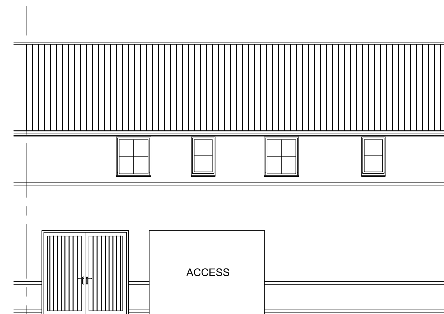
REAR ELEVATION
