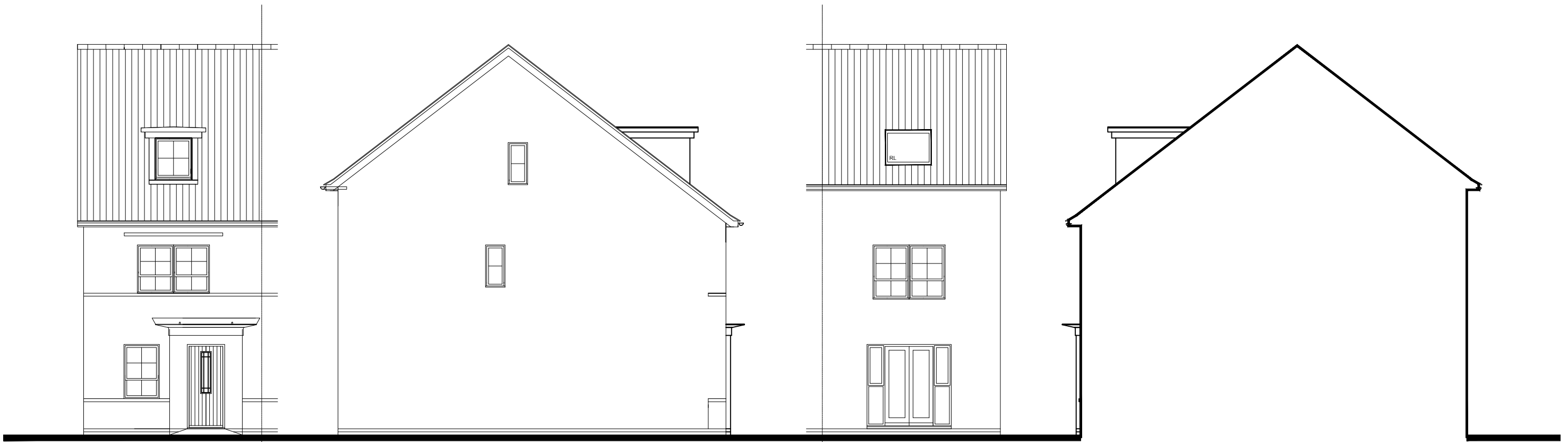
FRONT ELEVATION
