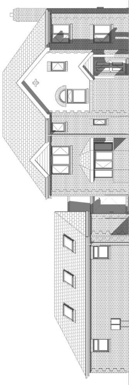
NE ELEVATION (FRONT)
