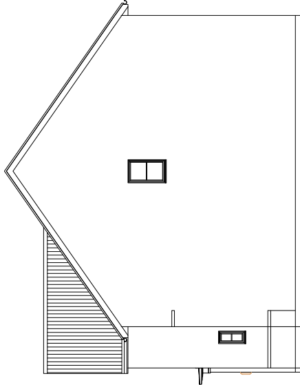
SIDE ELEVATION 1
