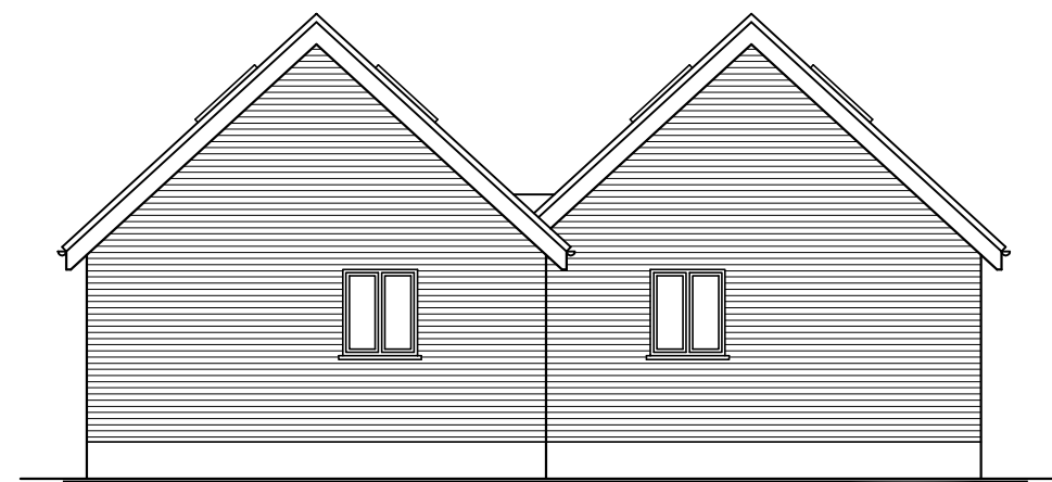
NORTH / SOUTH ELEVATIONS
