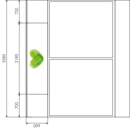
FASCIA 2 LAYOUT scale 1:50
