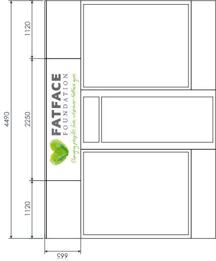
FASCIA 1 LAYOUT scale 1:50
