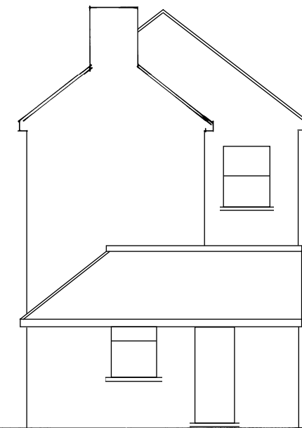
Existing East/Rear Elevation
