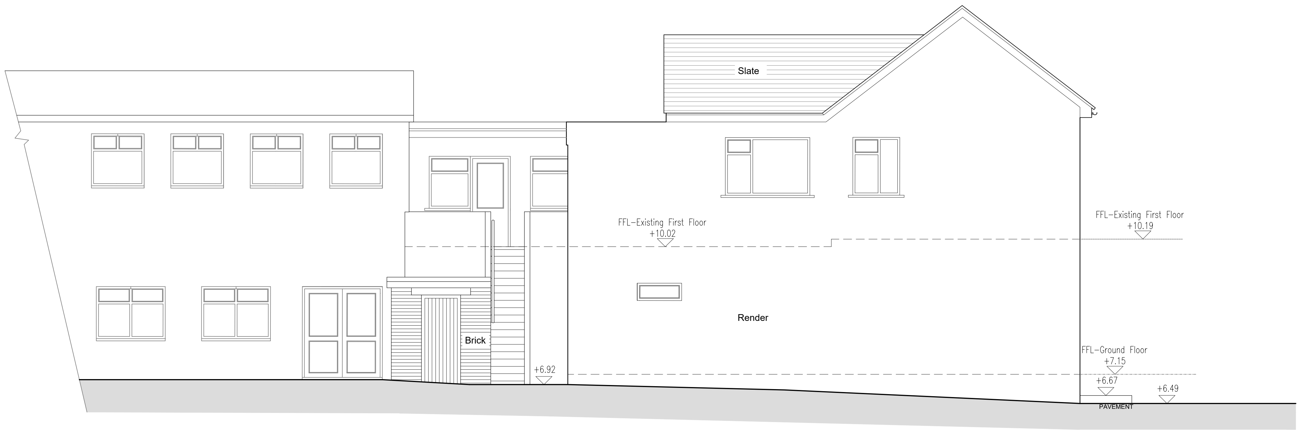
EXISTING BUSINESS UNIT EXISTING EAST ELEVATION
