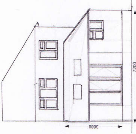
Proposed Rev Front Elevation 1:100
