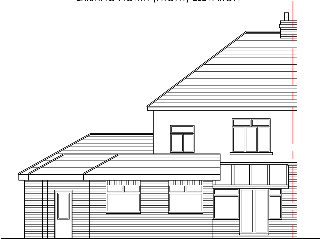
EXISTING SOUTH (REAR) ELEVATION
