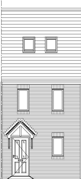
Front Elevation
