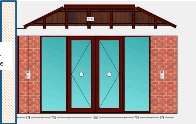
South Elevation
