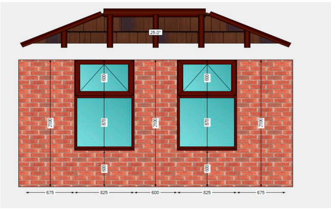
East Elevation
