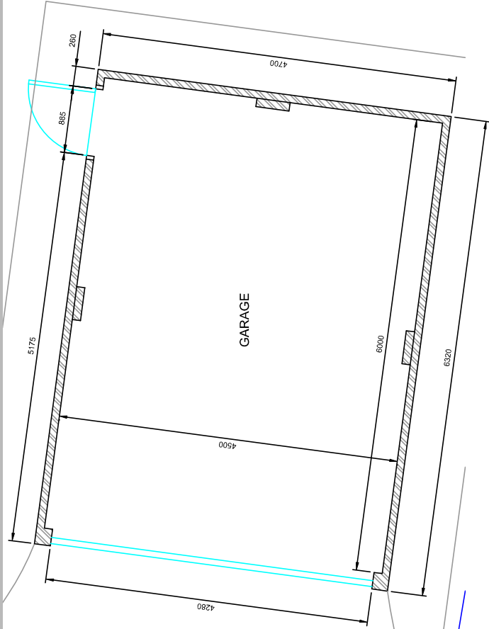
Floor plan SCALE @ A3: 1:50
