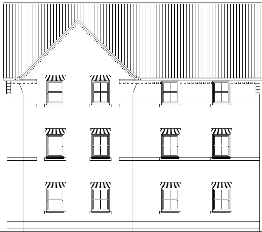
SIDE ELEVATION 1
