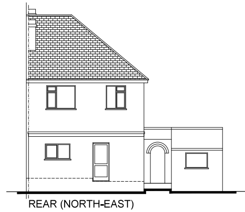
REAR (NORTH-EAST)
