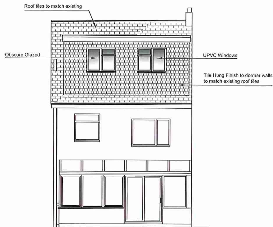
Rear Elevation
