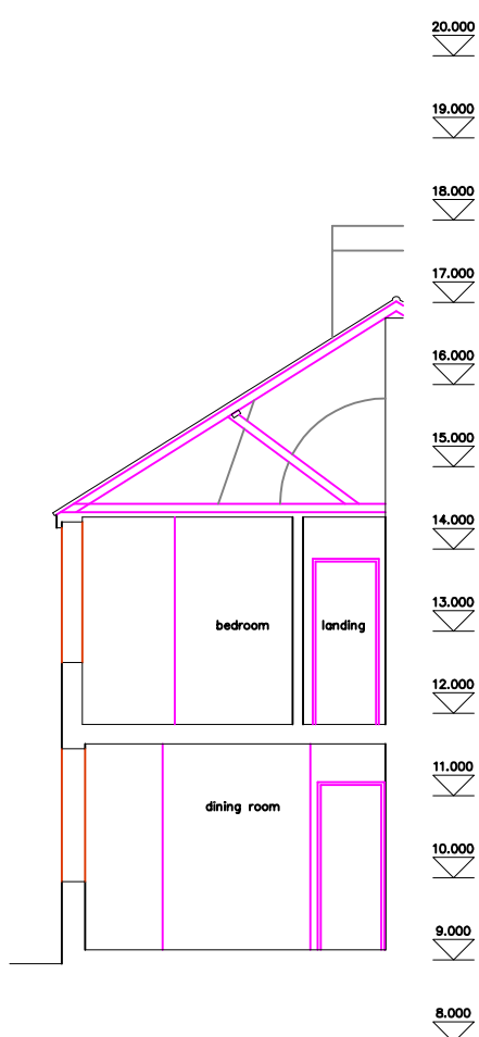
Section B-B 1:100
