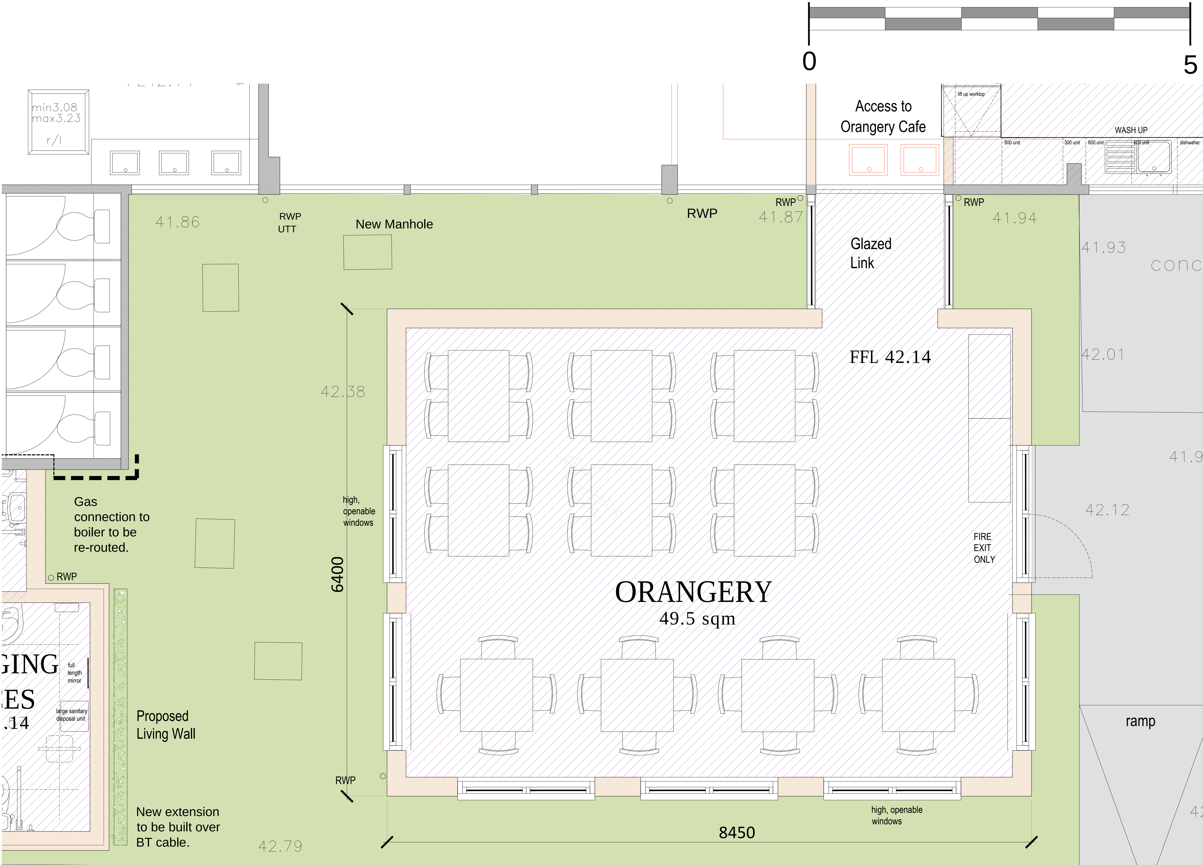
ORANGERY - PROPOSED LAYOUT
