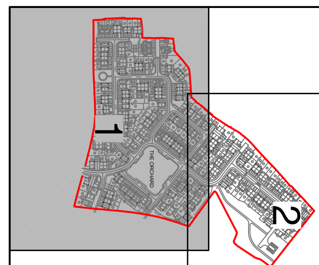
1:500 KEYPLAN
