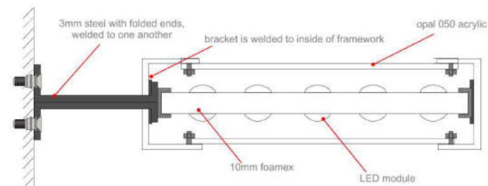
Steel bracket detail (plan view) Scale: NTS
