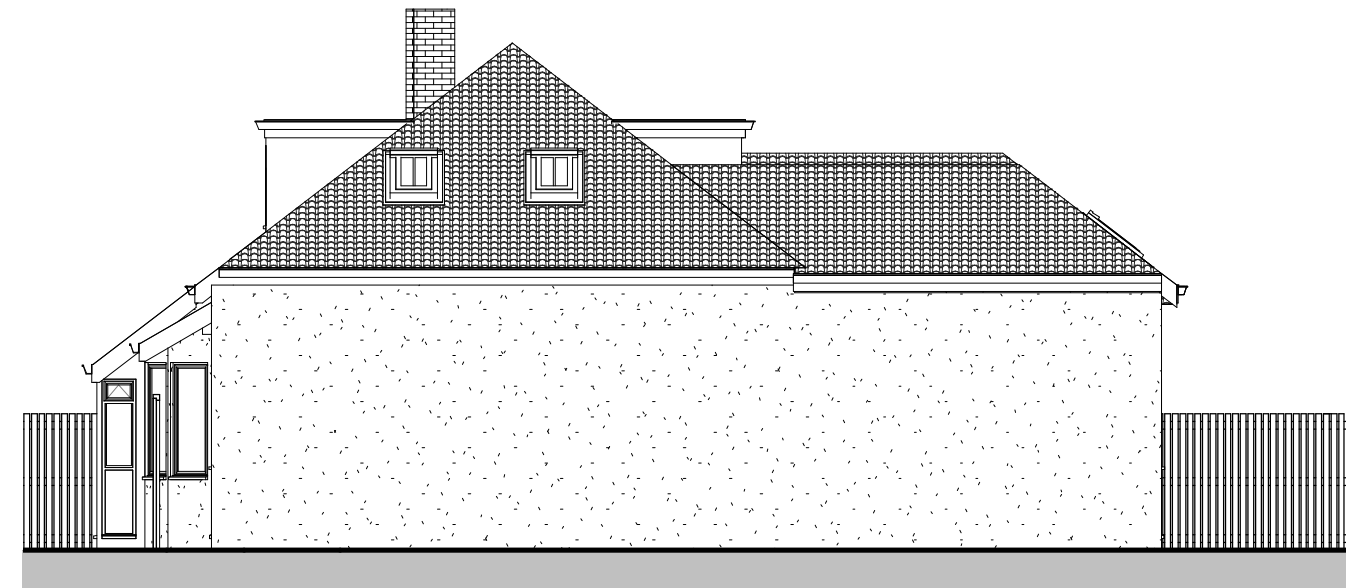
4 West Elevation 1 : 100
