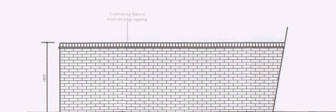
1800mm Brick Wall (Scale 1:50)
