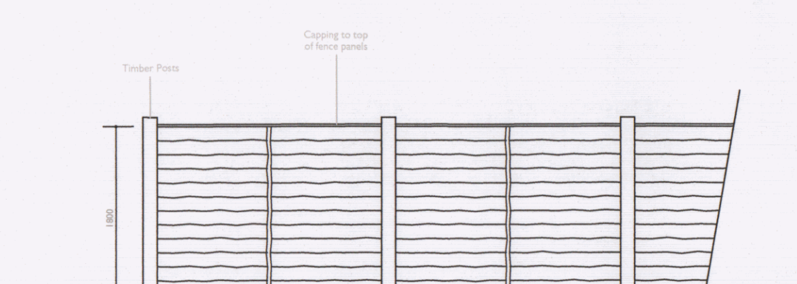
1800mm High Larch Lap Panel Fence (Scale 1:50)
