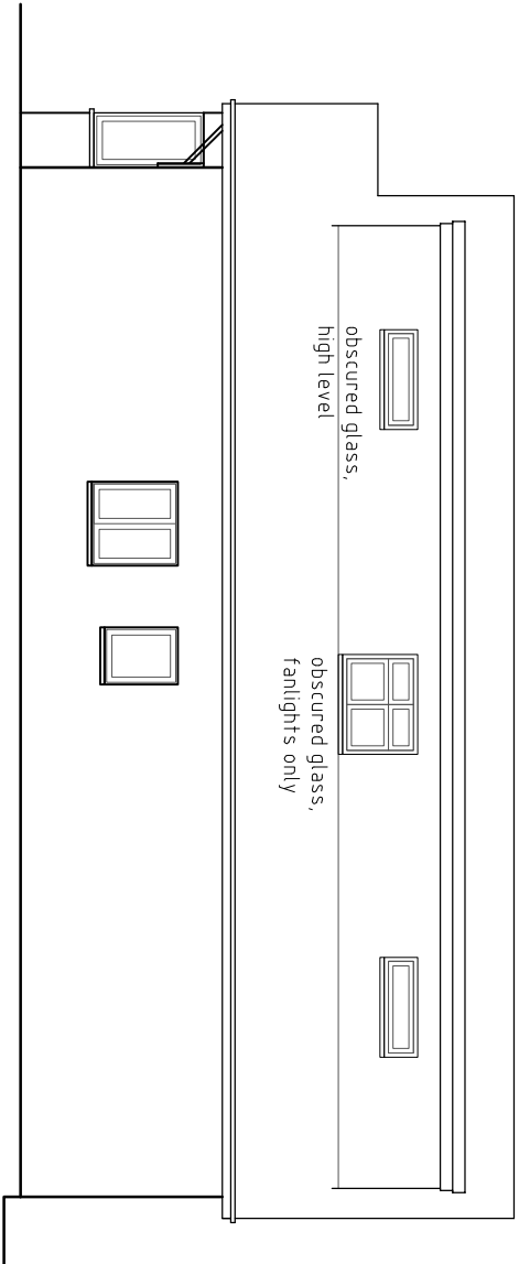
SIDE (SOUTH) 1:100
