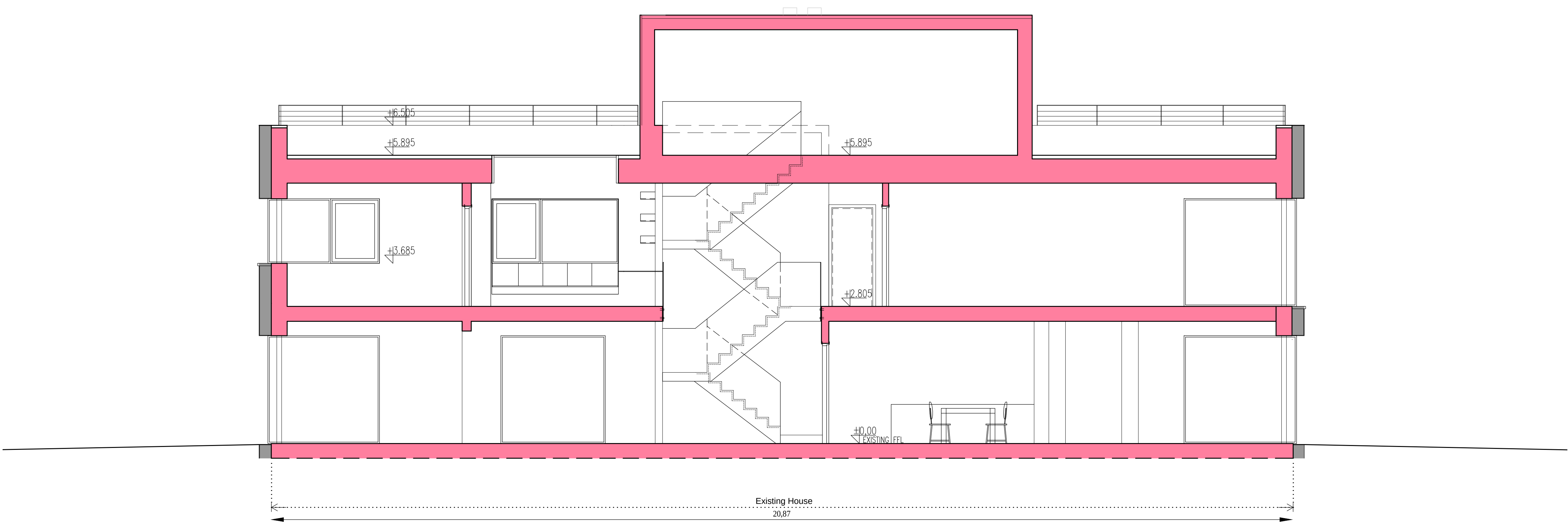
SECTION EE
