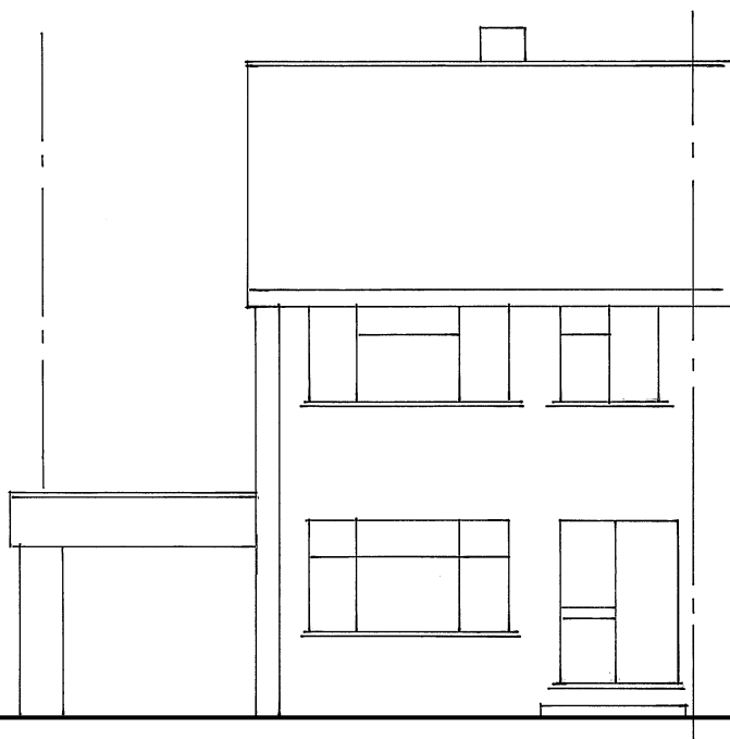
Existing South/Front Elevation
