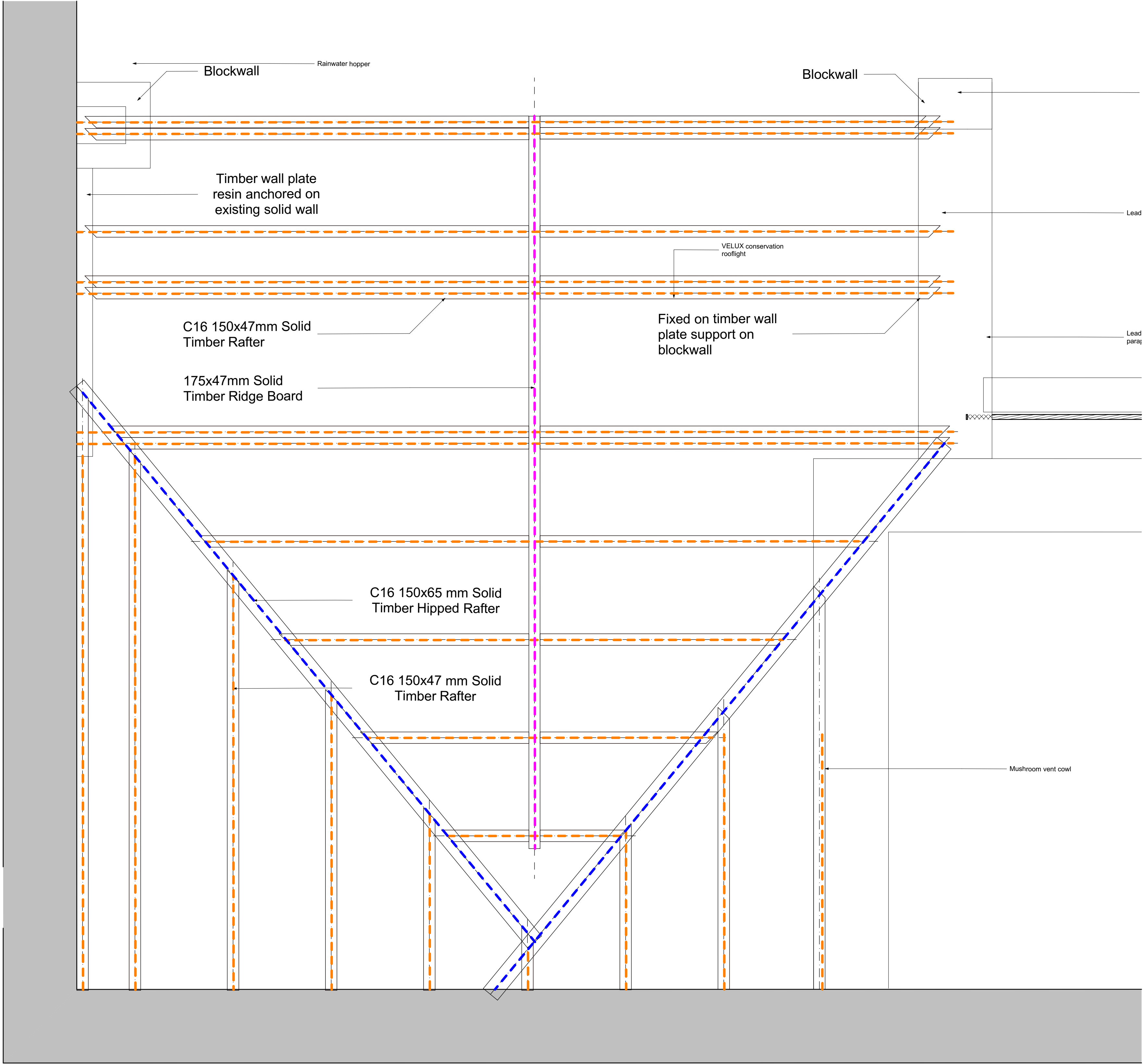
1:10 Plan - Roof structure layout
