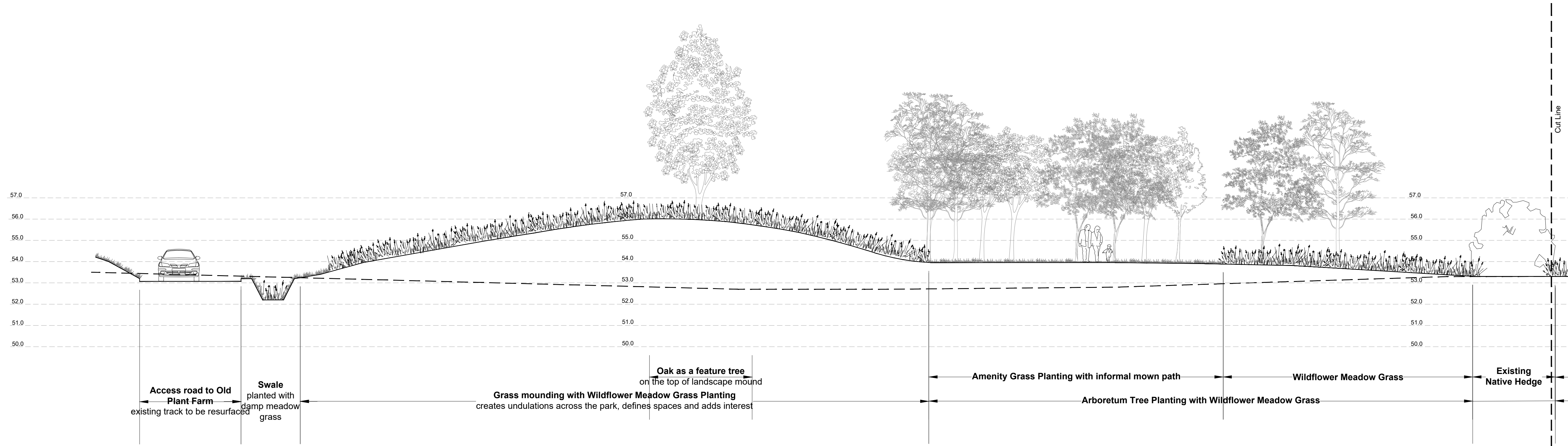
SECTION C-c
