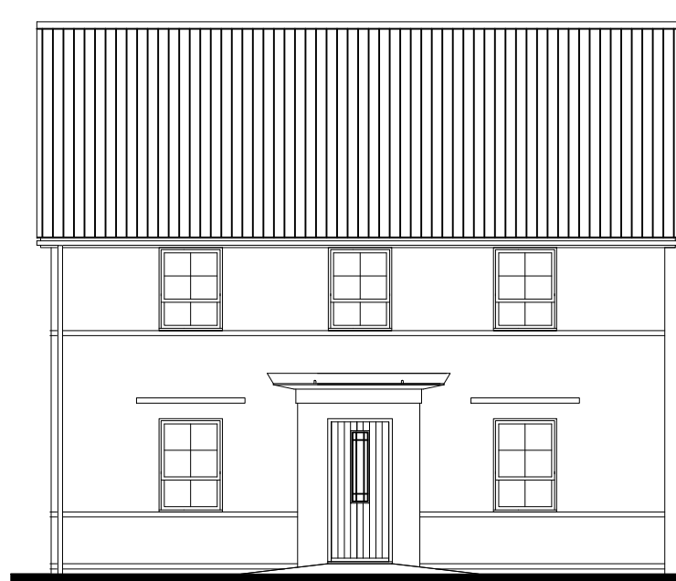
FRONT ELEVATION 1
