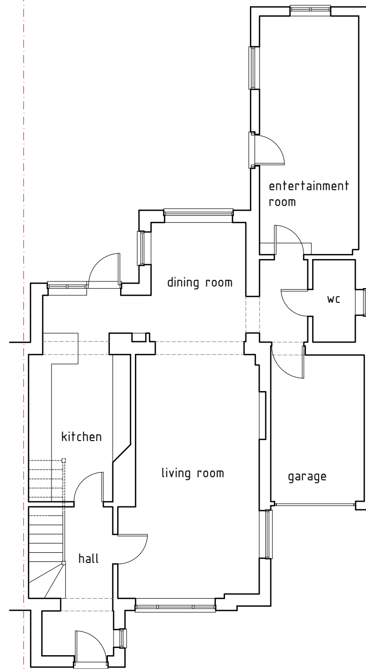
GROUND FLOOR LAYOUT
