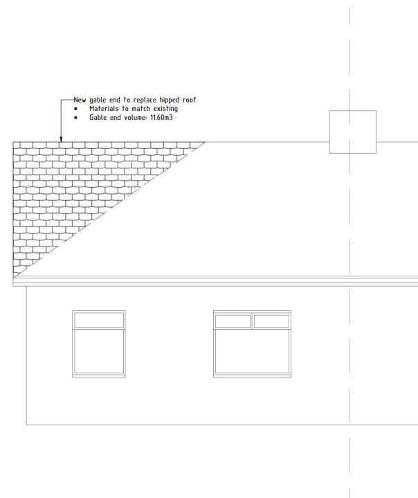
Elevation Facing East
